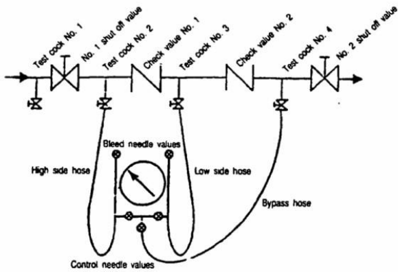
Figure 1—Double Check Value Assembly
